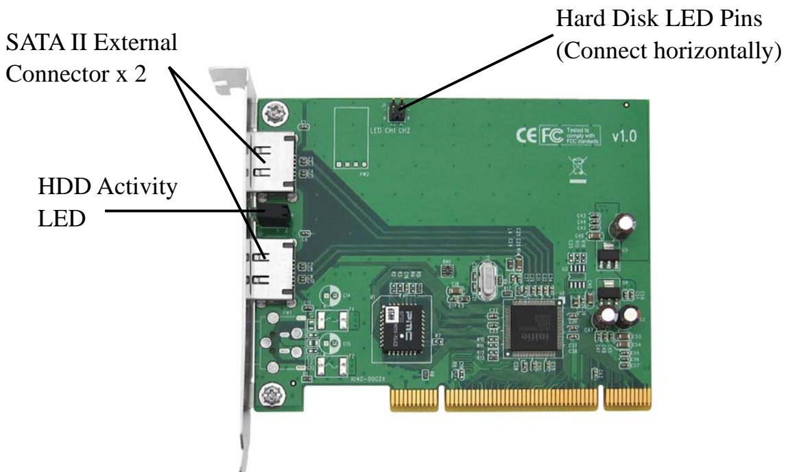
Figure 3. SATA II 2-ext.-channel RAID PCI
